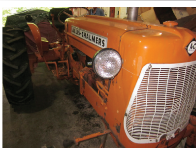
Allis-Chalmers D-15 tractor, gas powered, wide front
